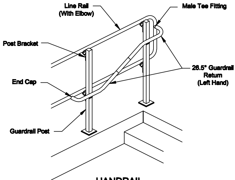
HANDRAIL MOUNTED TO GUARDRAIL
