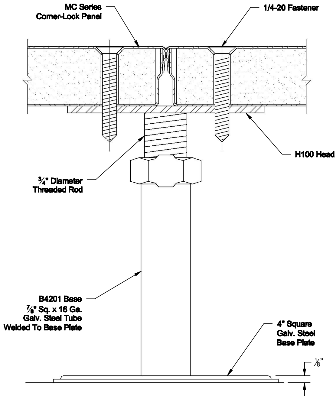
SIDE ELEVATION DETAIL
