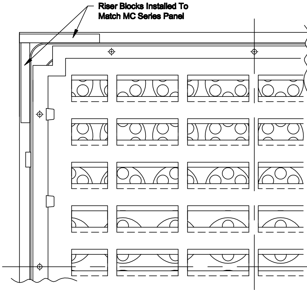
PARTIAL BOTTOM VIEW (Shown With Damper 75% Open)
