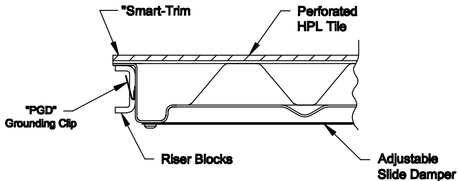
PARTIAL SECTION VIEW
