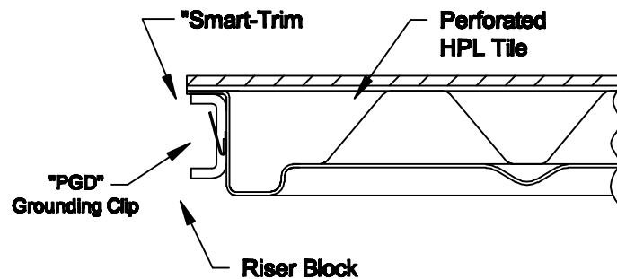
PARTIAL SECTION VIEW
