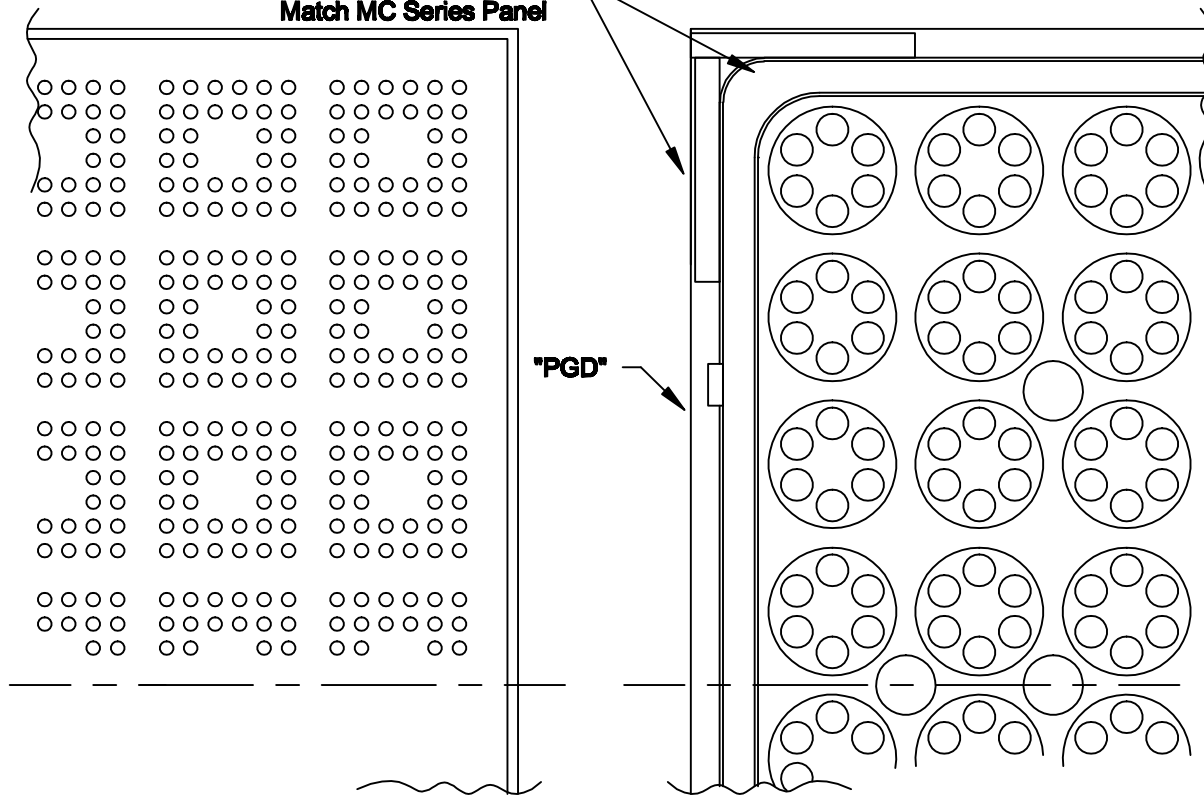
Riser Blocks Installed To Match MC Series Panel
