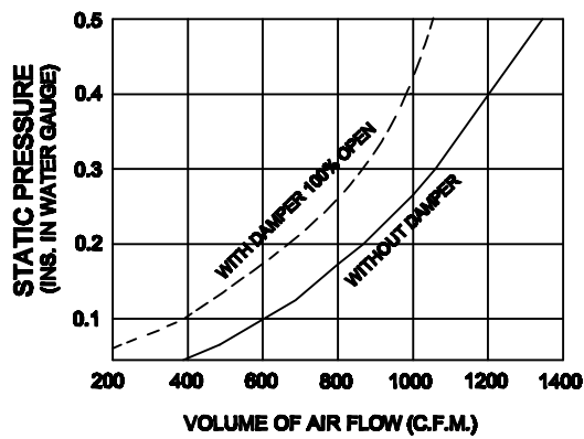
AIR FLOW CHARACTERISTICS
