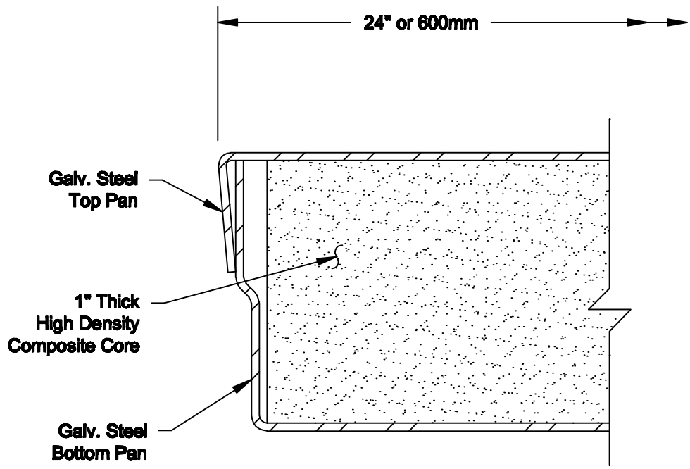
ENLARGED SECTION VIEW
