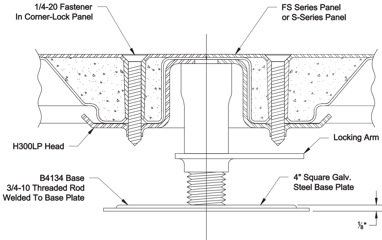
SIDE ELEVATION DETAIL
