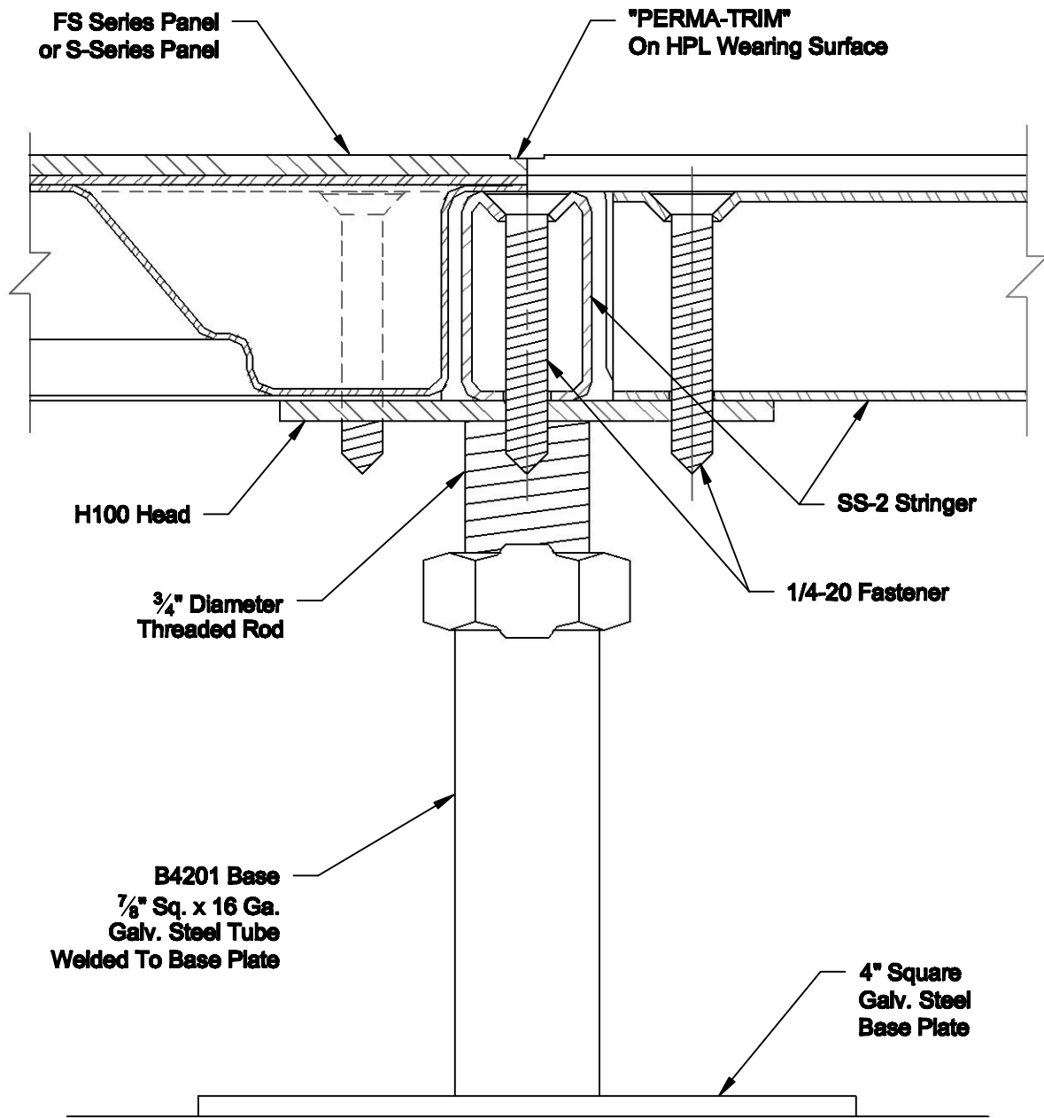
SIDE ELEVATION DETAIL
