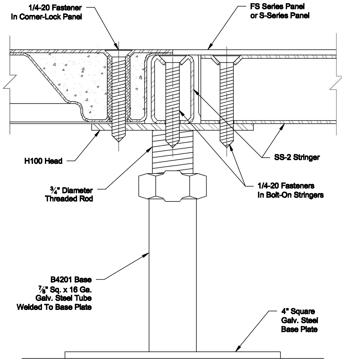
SIDE ELEVATION DETAIL
