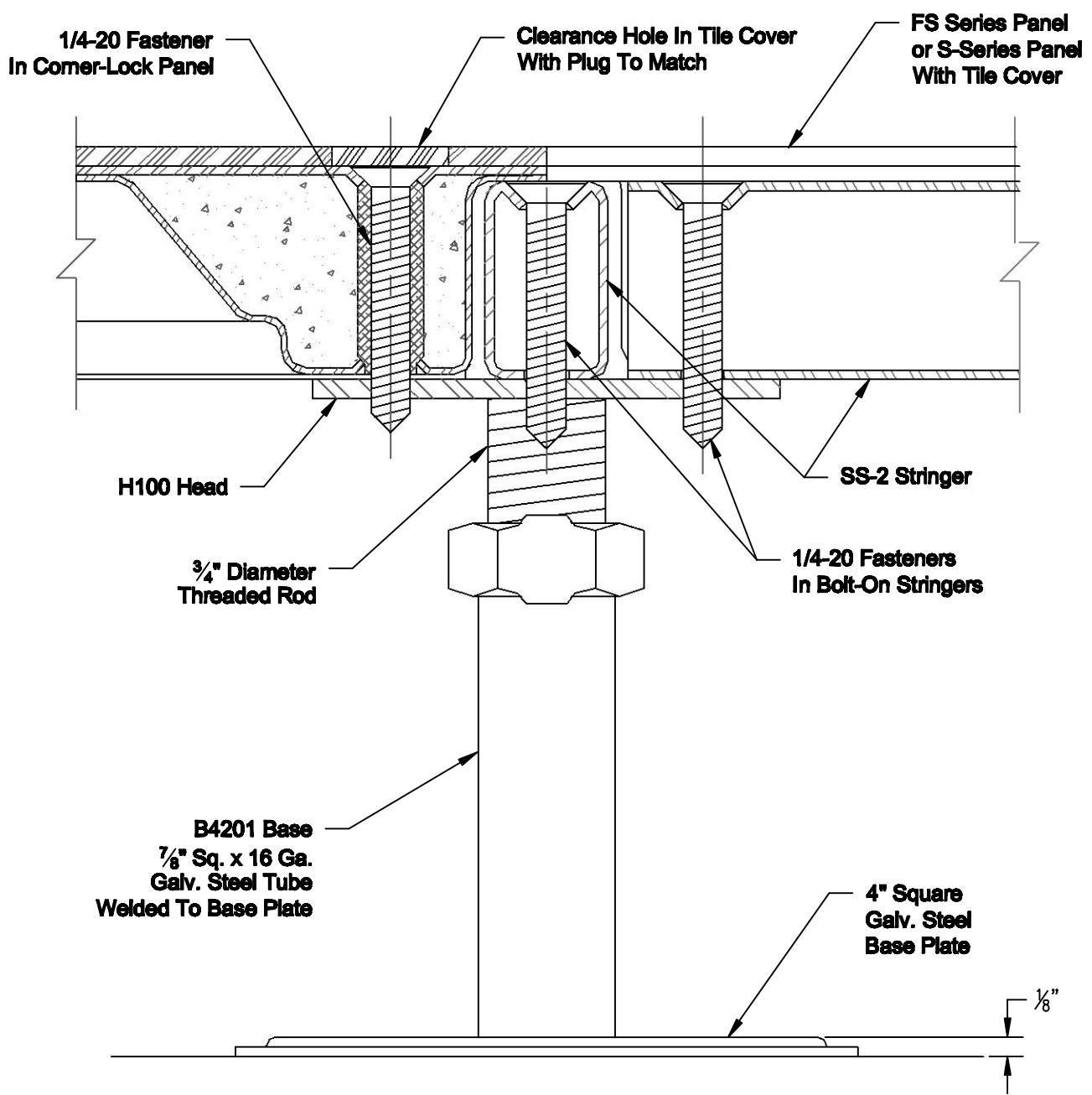
SIDE ELEVATION DETAIL
