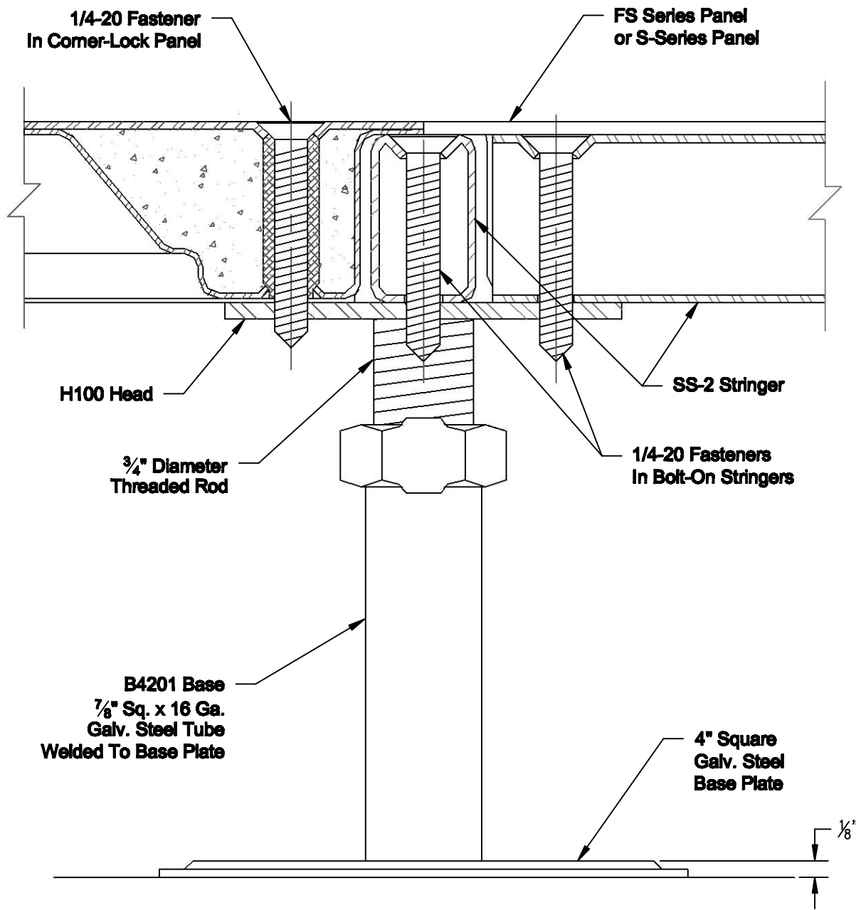
SIDE ELEVATION DETAIL
