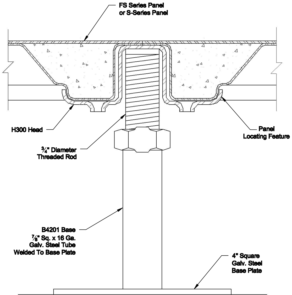
SIDE ELEVATION DETAIL
