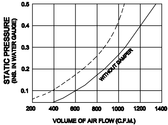
AIR FLOW CHARACTERISTICS
