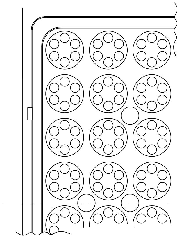
PARTIAL BOTTOM VIEW (Shown Without Optional Damper)
