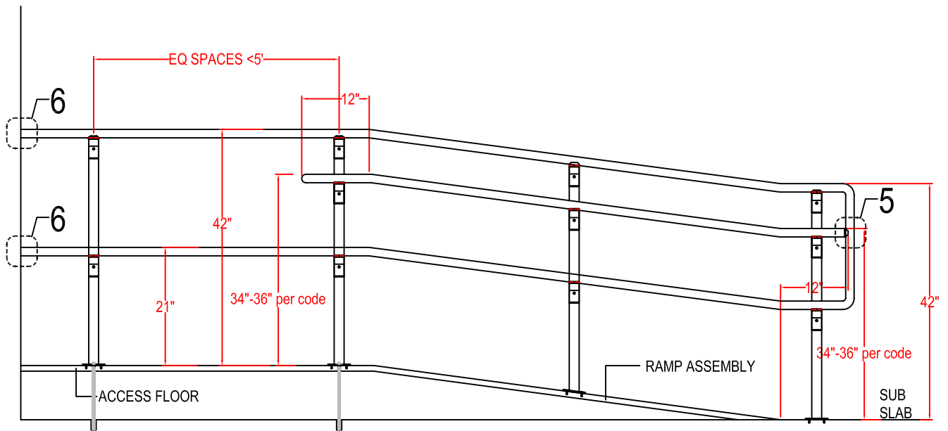
ELEVATION VIEW OPEN RAMP
