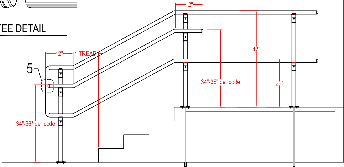
ELEVATION VIEW OPEN STEP
