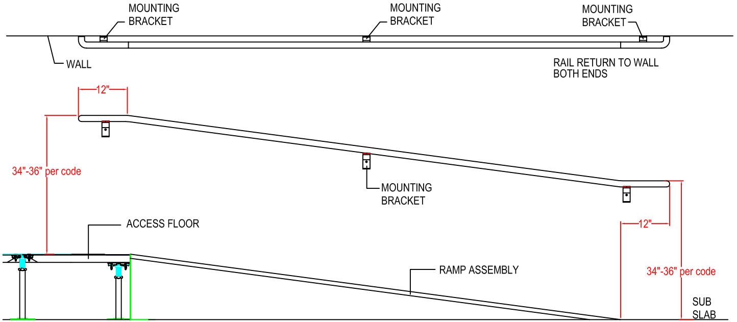
ELEVATION VIEW RAMP WALL MOUNT
