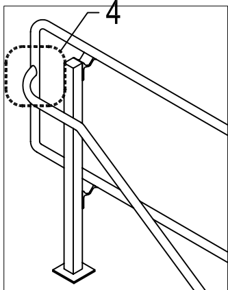
3 TEE DETAIL
